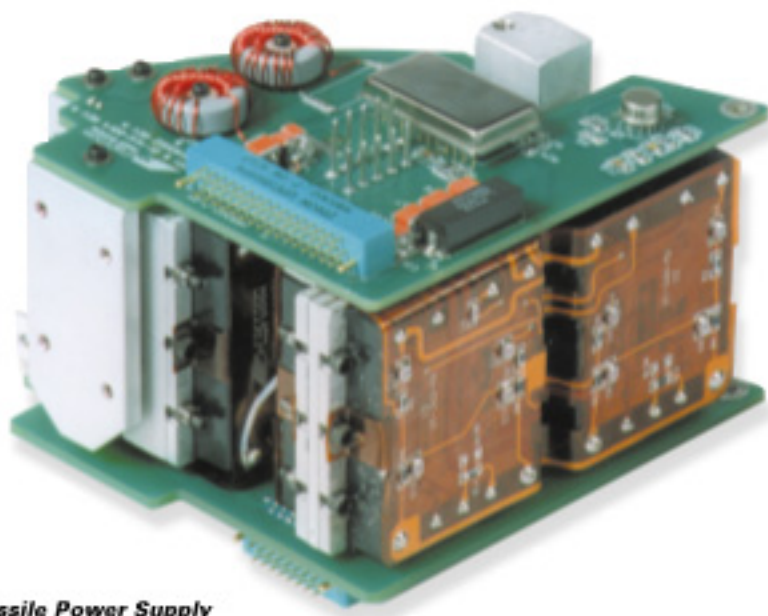
F-2012: Multiple Output Missile Power Supply
